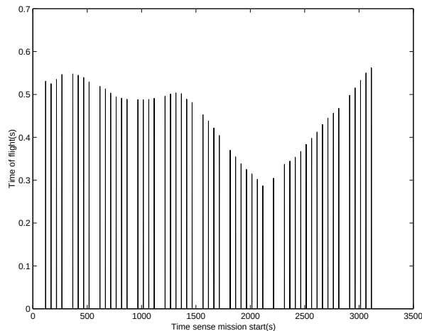
Figure 5. Returns from LBL transponder 1
