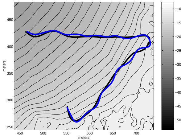
Figure 4. Results showing the LOST2 system performance. The origin is at (602500,4739293) UTM. LOST2's estimated vessel track is the solid blue line, and the INS/LBL generated position is the solid black line.
