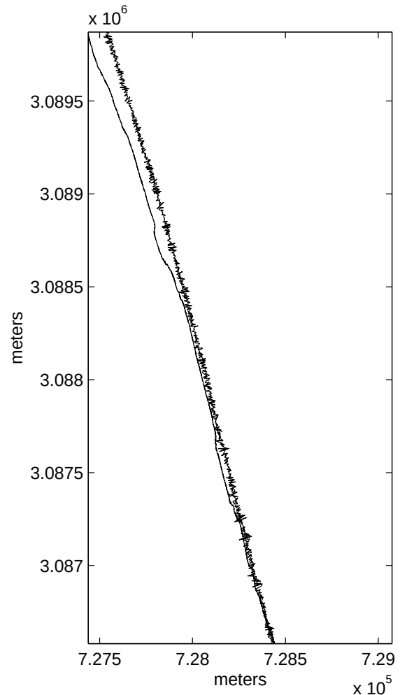
Figure 2. A close up of a run with a start-up transient. The dotted, fuzzy line is the USBL position and the solid line that starts to the left and converges with the USBL position is the LOST2 position estimate
