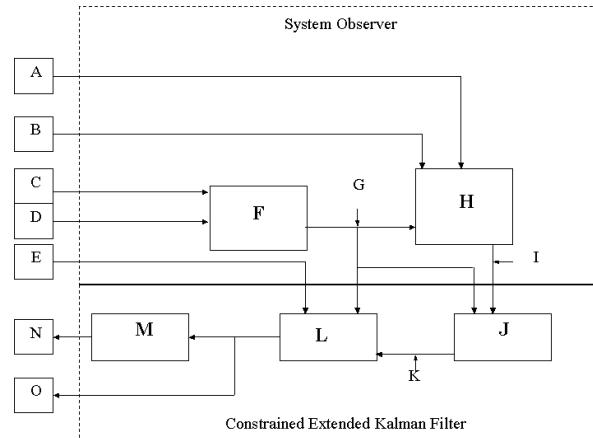
Figure 1. Block diagram of the LOST2 system showing its two primary subsystems and the system inputs and outputs. A - High Resolution Bathymetry, B -Vessel's measured ocean depth, C - Vessel's predicted state using all information before current time step, D - Vessel's measured velocity, E - Measured slant range and location of known point, F - State velocity update Module, G - Vessel's final predicted position, H - Terrain matching module, I - Terrain based position estimate, J - Steady state Kalman Filter, K- Linear filter's position estimate, L - Non-linear constraints module, M - State Predictor module, N - Vessel's predicted position at next time step using all current information, O - Vessel's final estimated position
