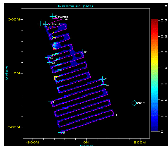
Figure 6: Full Field Run and Plume Data
