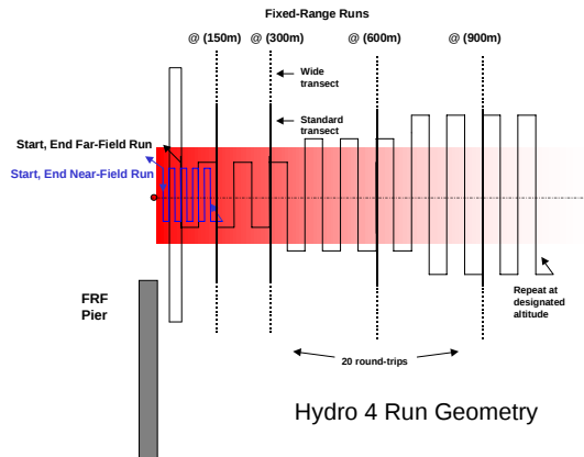
Figure 3: Types of REMUS runs [Morris 2001]
