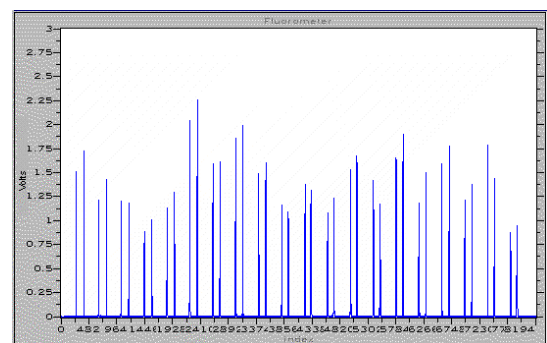
Figure 5: Fixed range plume data showing time variation of dye concentration with each successive crossing.
