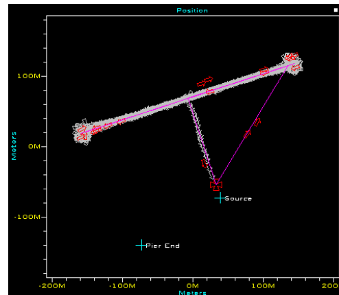
Figure 4: Fixed Range Run
