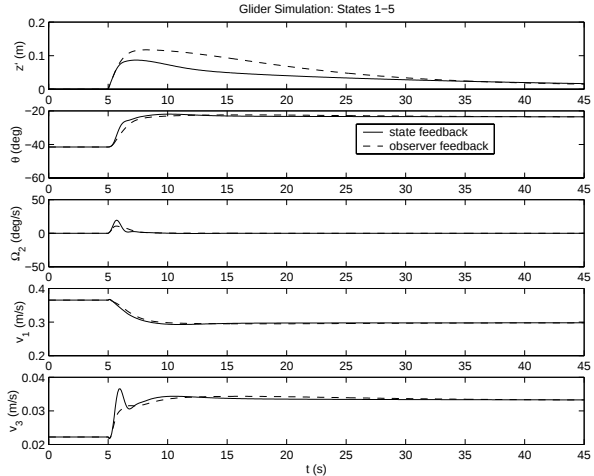
Figure 5.2: Simulation of position and velocity variables.
