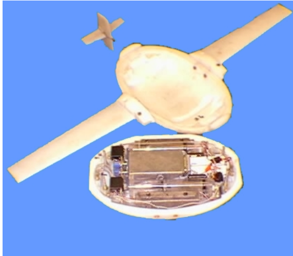
Figure 2.1: ROGUE with hull open.
