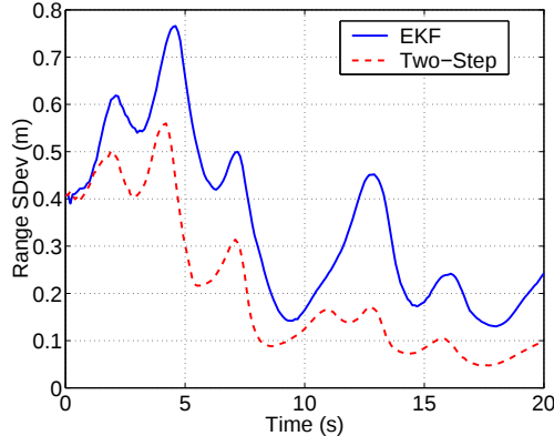
Figure 9: Monte Carlo Standard Deviation for Range
