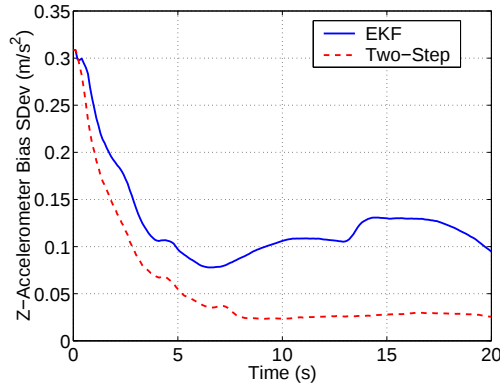
Figure 10: Monte Carlo Standard Deviation for Z-Accelerometer Bias
