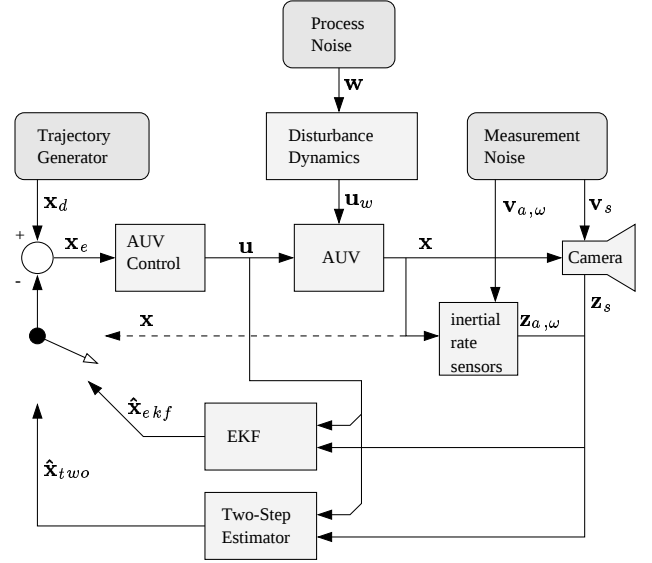
Figure 2: Block Diagram with AUV Controller, Sensors, and Estimators
