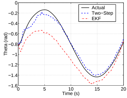
Figure 8: Theta Estimate
