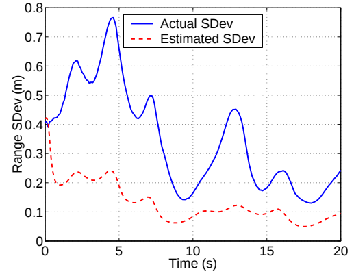
Figure 13: Comparison of Standard Deviation for the Range coordinate of the EKF
