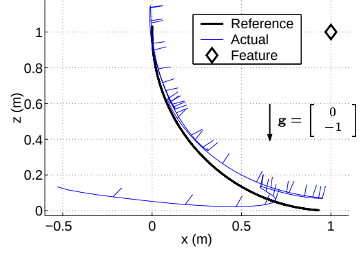
Figure 4: A 2D Simulation showing the Actual and Reference Trajectory and the Visual Feature
