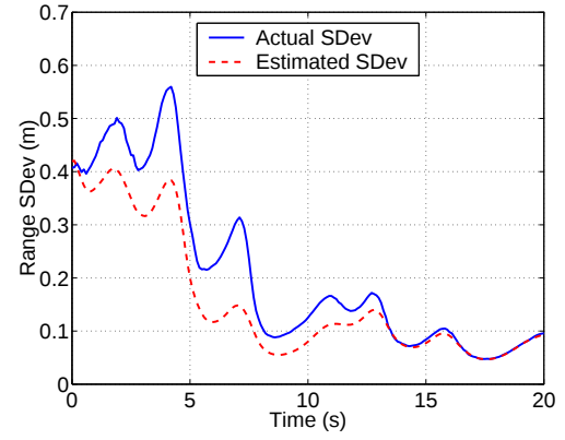
Figure 12: Comparison of Standard Deviation for the Range coordinate of the Two-Step Estimator
