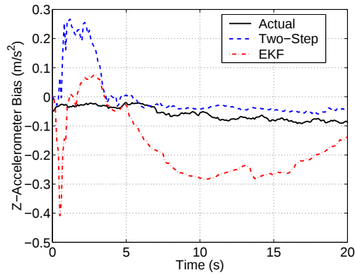
Figure 7: Z-Accelerometer Bias Estimate
