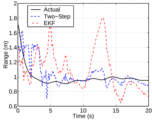
Figure 6: Range Estimate
