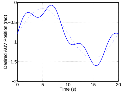
Figure 5: Desired AUV Position Expressed as an Angle along an Arc
