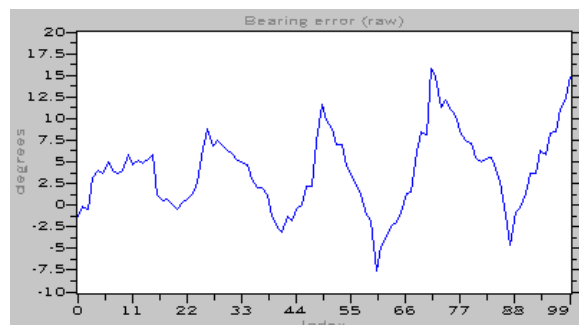
Fig. 6. Calculated deviations with transponder adrift
