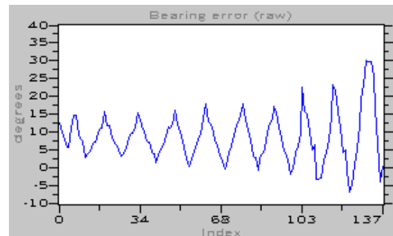
Fig. 7. Misplaced transponder errors
