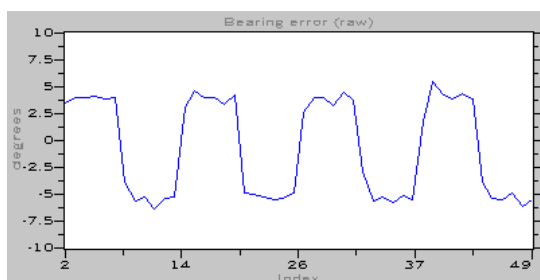
Fig. 3. Bearing error for typical survey mission
