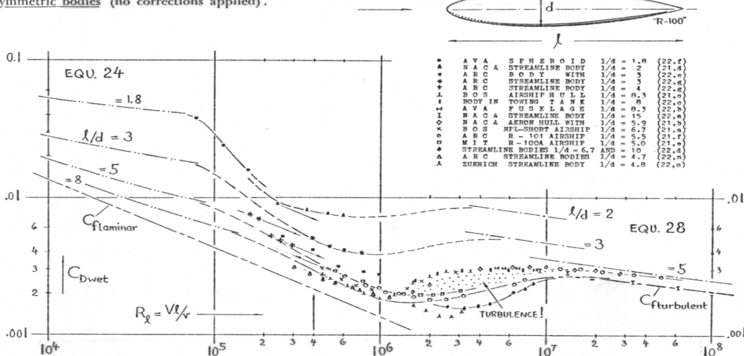
Figure 22. Selected results on the drag of rotationally-symmetric bodies (no corrections applied).
