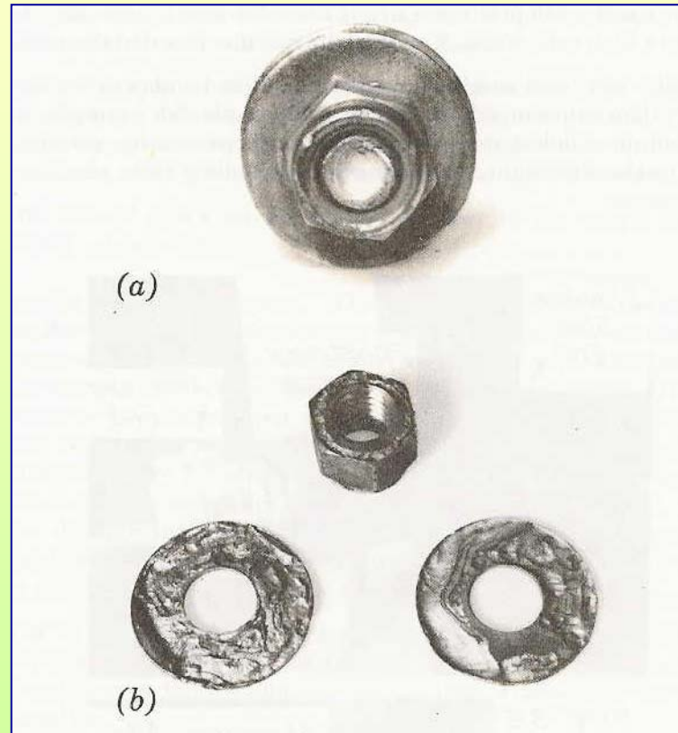
Crevice corrosion
