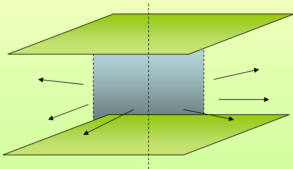
Ducts: Cylindrical Spreading
