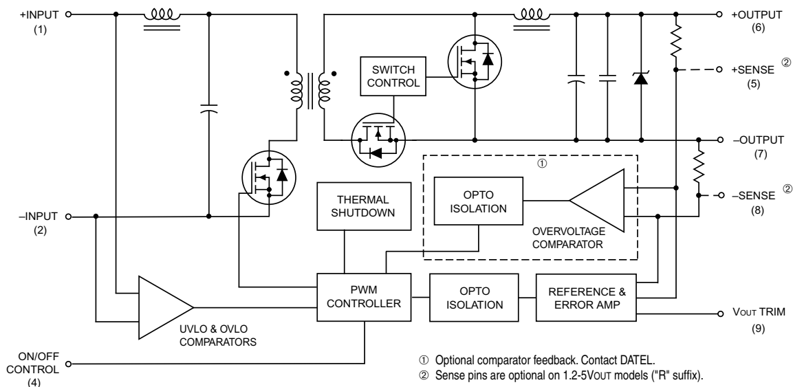
Figure 1. Simplified Schematic
