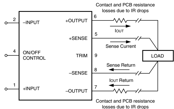
Figure 9. Remote Sense Circuit Configuration
