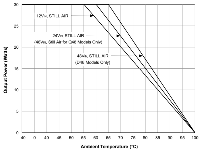
UHE-12/2500 and UHE-15/2000 (All Models) Temperature Derating
