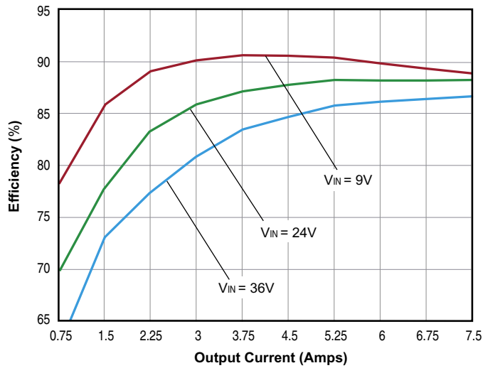
UHE-3.3/7500-Q12 Efficiency vs. Load @ +25°C Ambient
