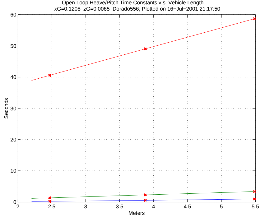
Figure 6: Stability Versus Length for Fixed Ring Area
