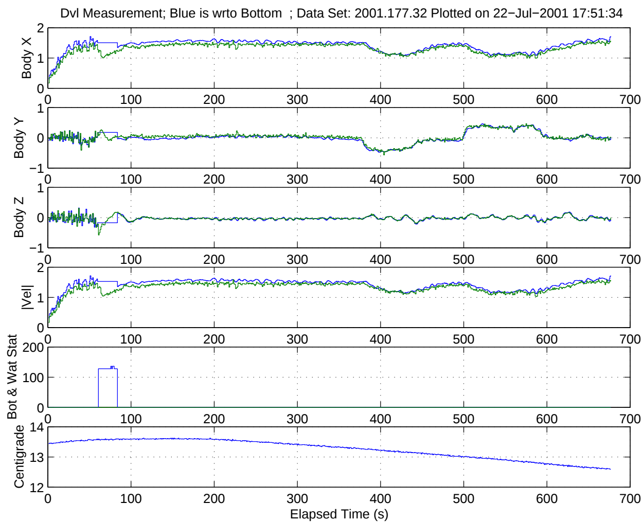
Figure 19: \vec{v}^{DVL_o} Measured by the DVL
