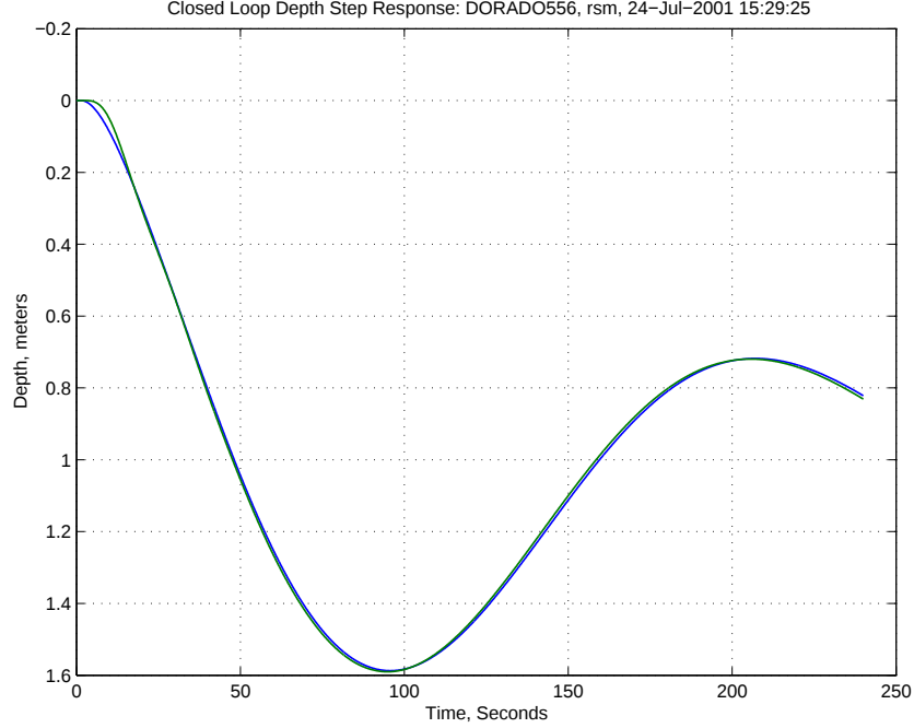
Figure 10: Depth Step Response of the Linearized Closed-Loop System
