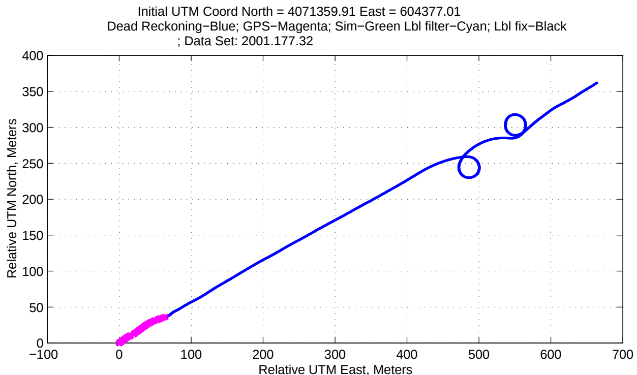
Figure 14: Ground Track
