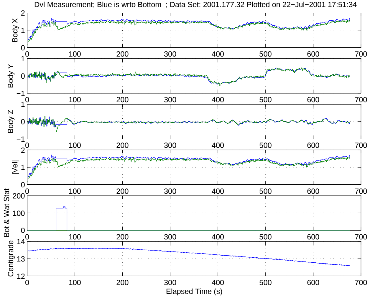
Figure 19: \vec{v}^{DVL_o} Measured by the DVL
