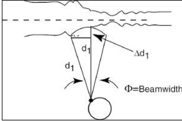
Figure 3: Schematic representation of the effect of beamwidth. Note that the sonar system records the first return that may not be directly above the vehicle.
