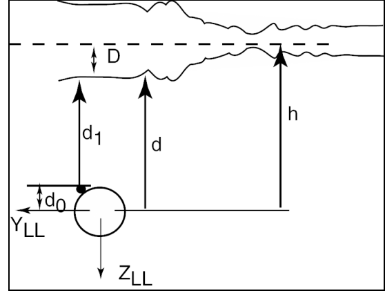
Figure 2: Schematic representation of the measurement of ice draft (D) from observations of distance from the transducer and depth of the vehicle (h).
