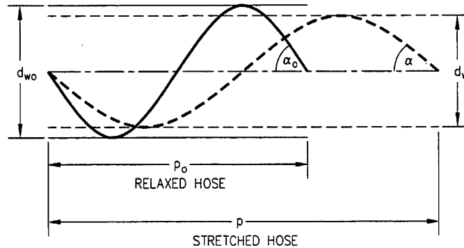
Figure 5: Side view of relaxed and elongated stretch hose
