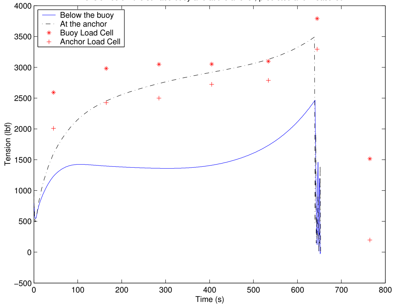
Tension below the surface buoy and at the anchor, predicted and measured
