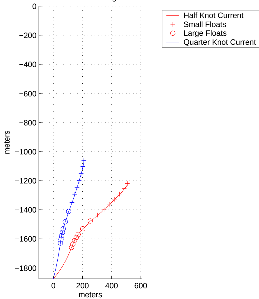
Bottom section of MOOS mooring in various currents
