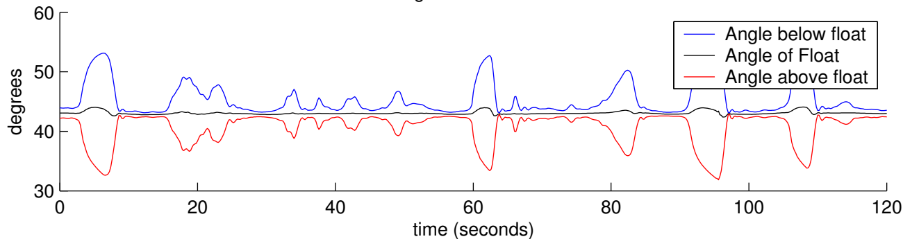
Bend-angle Results at Float #16
