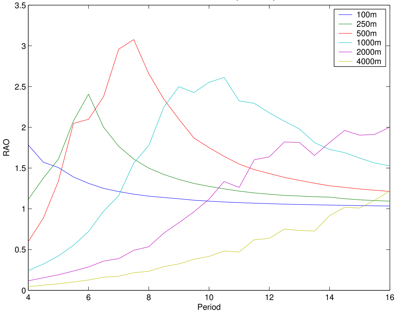
BIN motion relative to 1 meter amplitude ship motion
