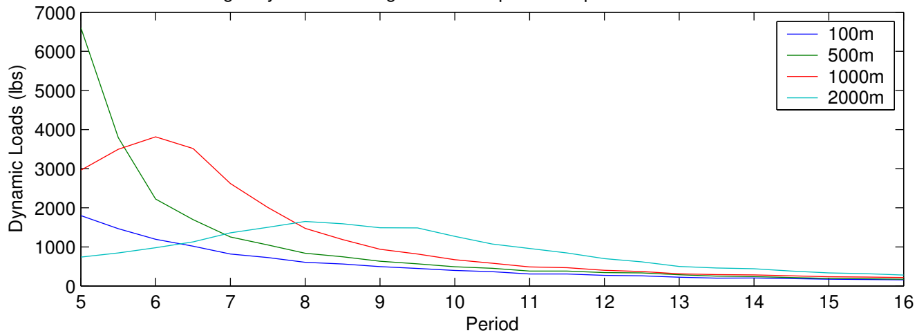
Fig2: Dynamic Loading and BIN amplitude response for 3/8" 3x19 wire
