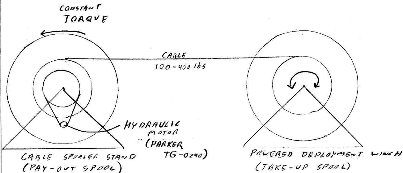
FIGURE 1: SCHEMATIC OF CABLE LOADING ONTO DEPLOYMENT WINCH.
