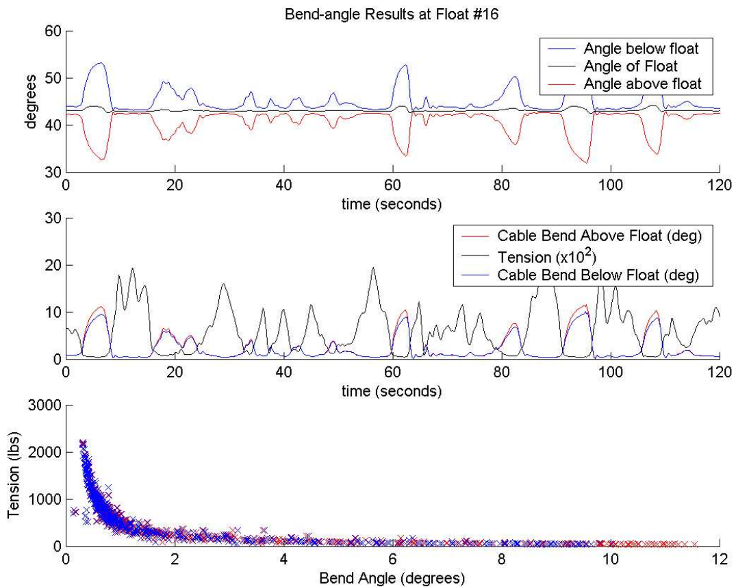
Figure 2: Cable bending at float location, 3 meter significant wave height.
