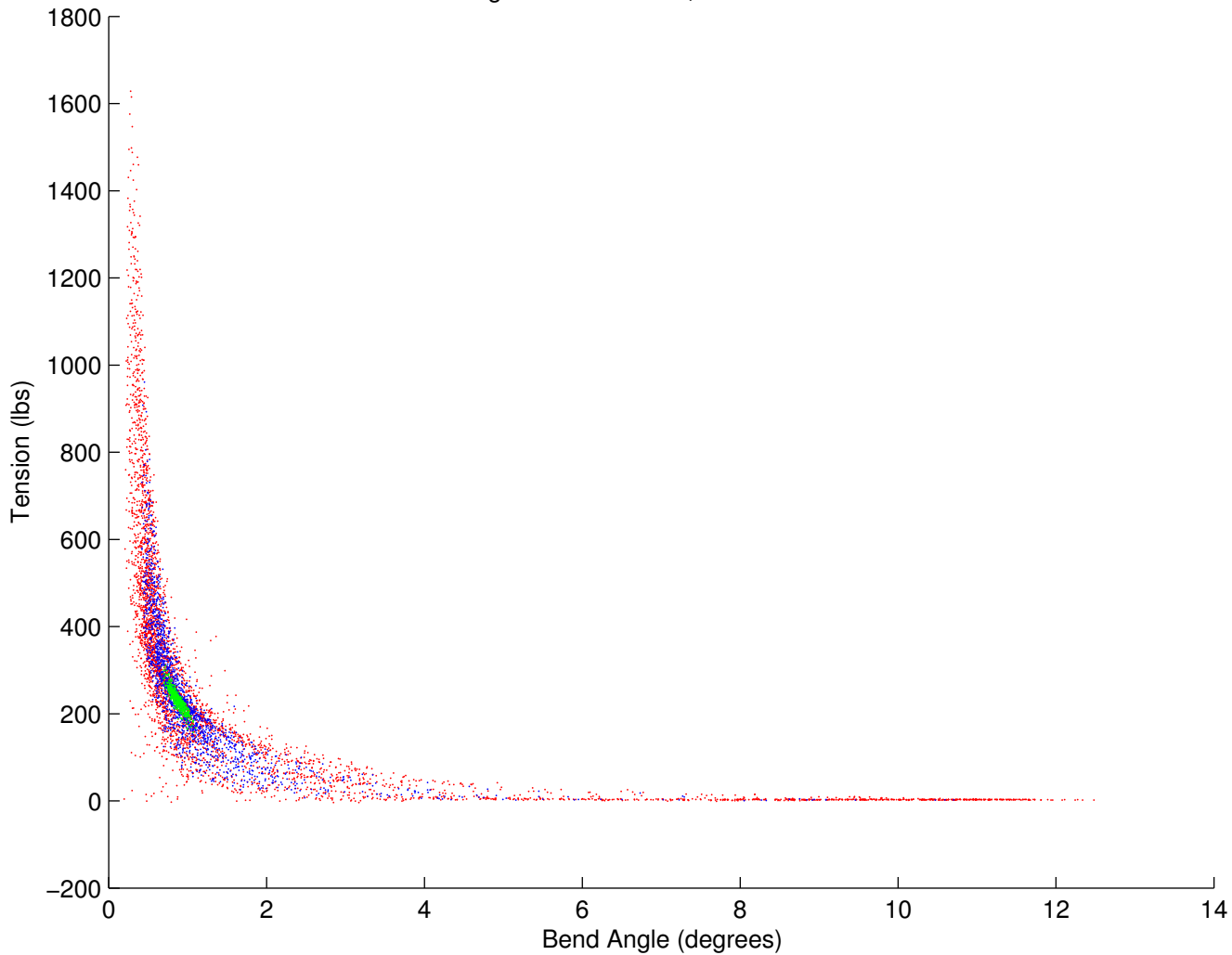
Bend Angle versus tension, above bend restrictor
