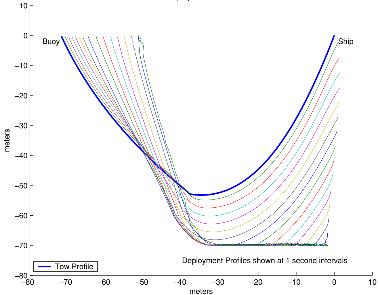
Tow and Deployment Profile at 2 knots
