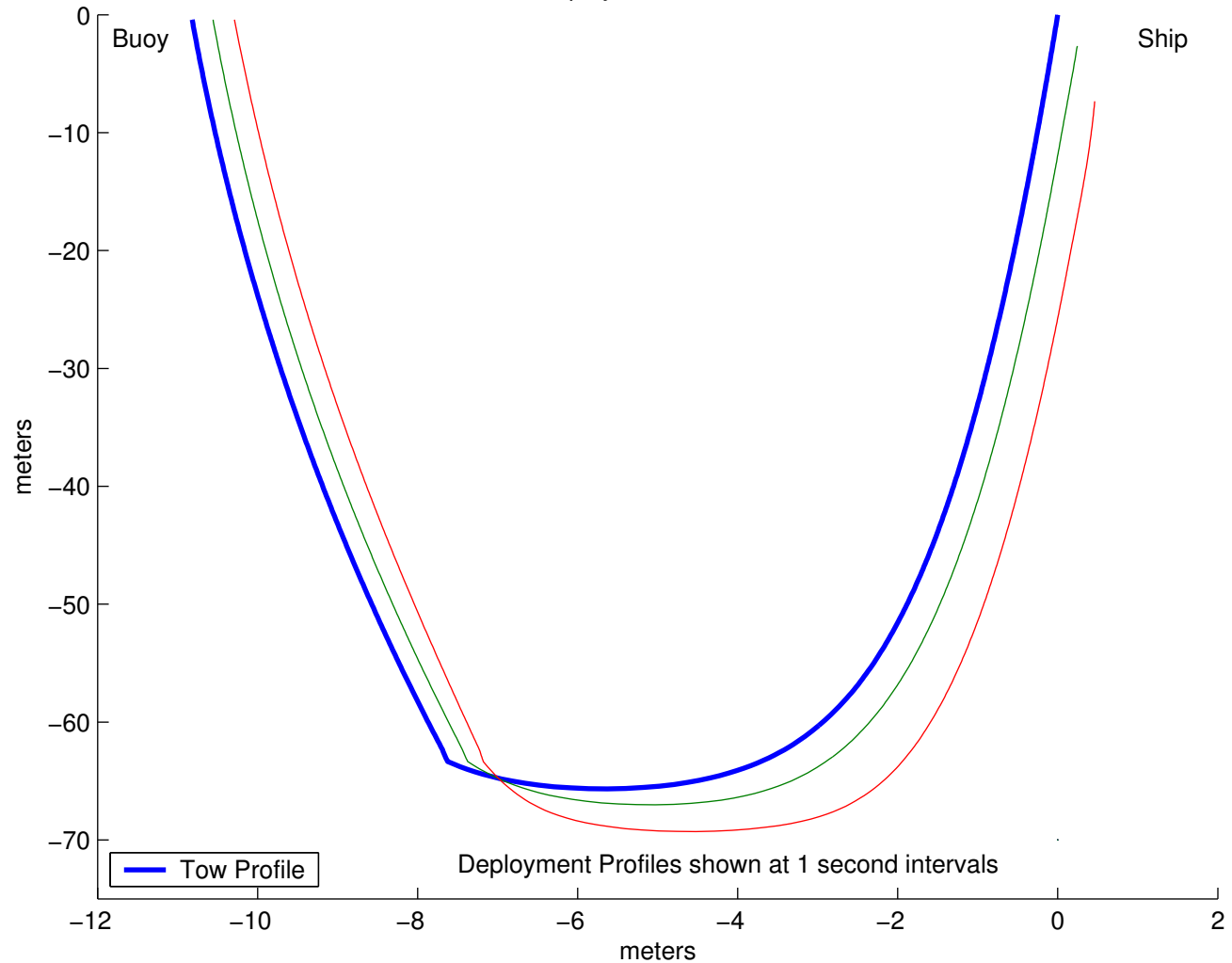
Tow and Deployment Profile at 0.5 knots
