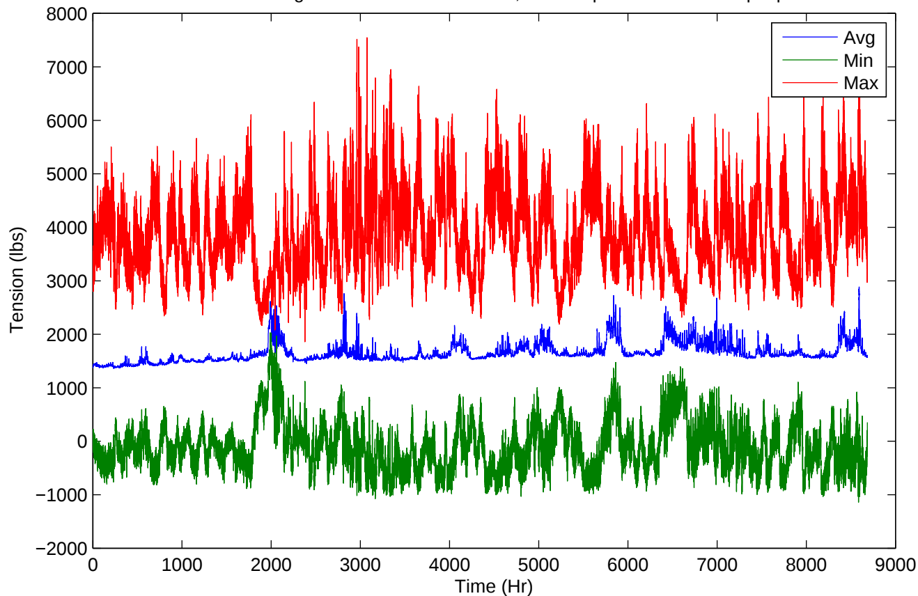
MTM-4 Mooring Tensions. 1 Year Record, Results per 10 minute sample period
