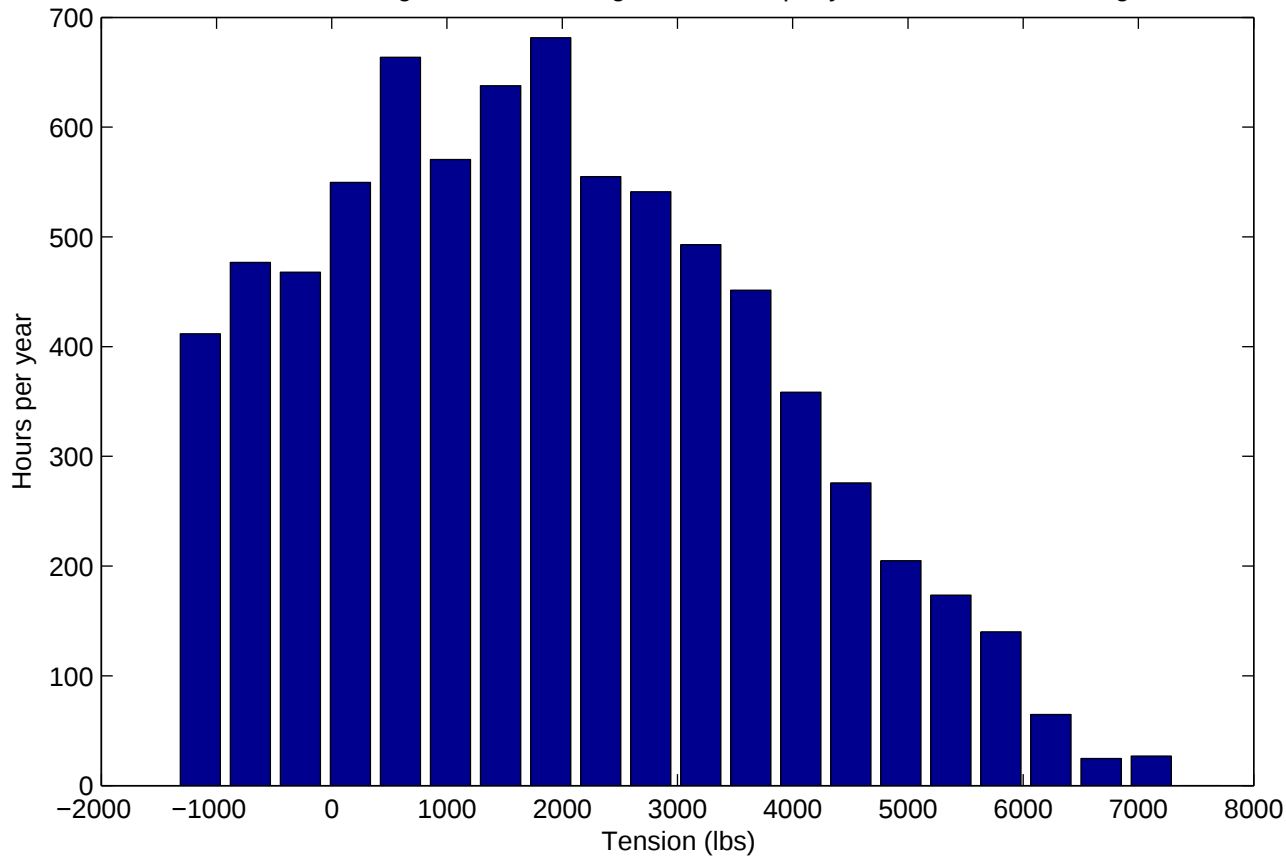
MTM-4 Mooring Tensions. Histogram of hours per year at each tension range
