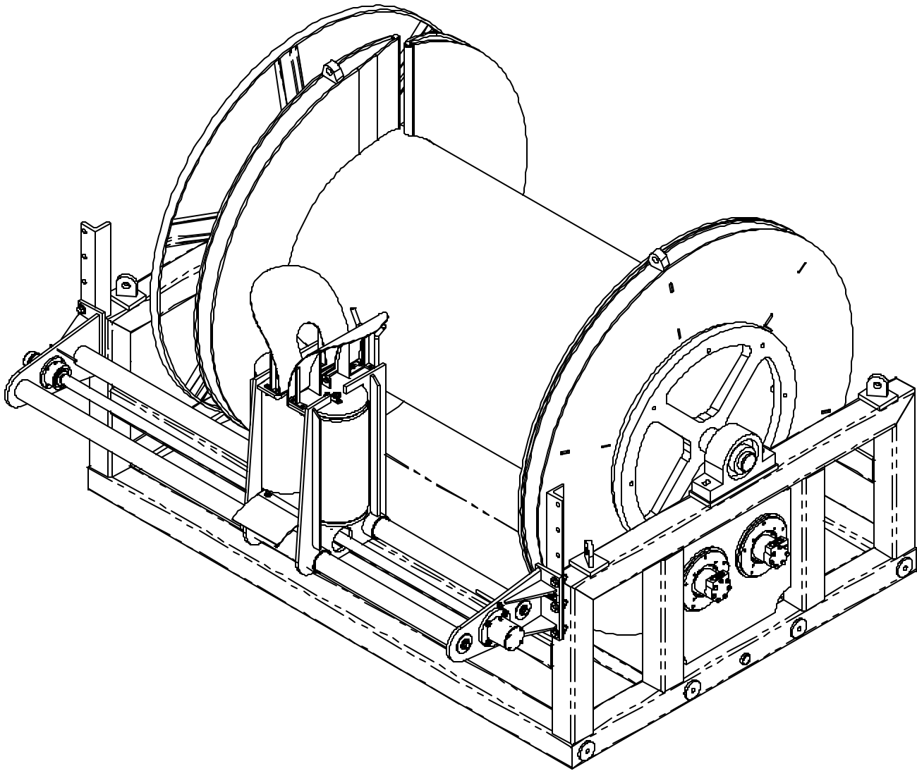
ISOMETRIC VIEWS
