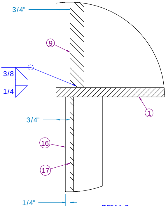
DETAIL B SCALE 1 : 3
