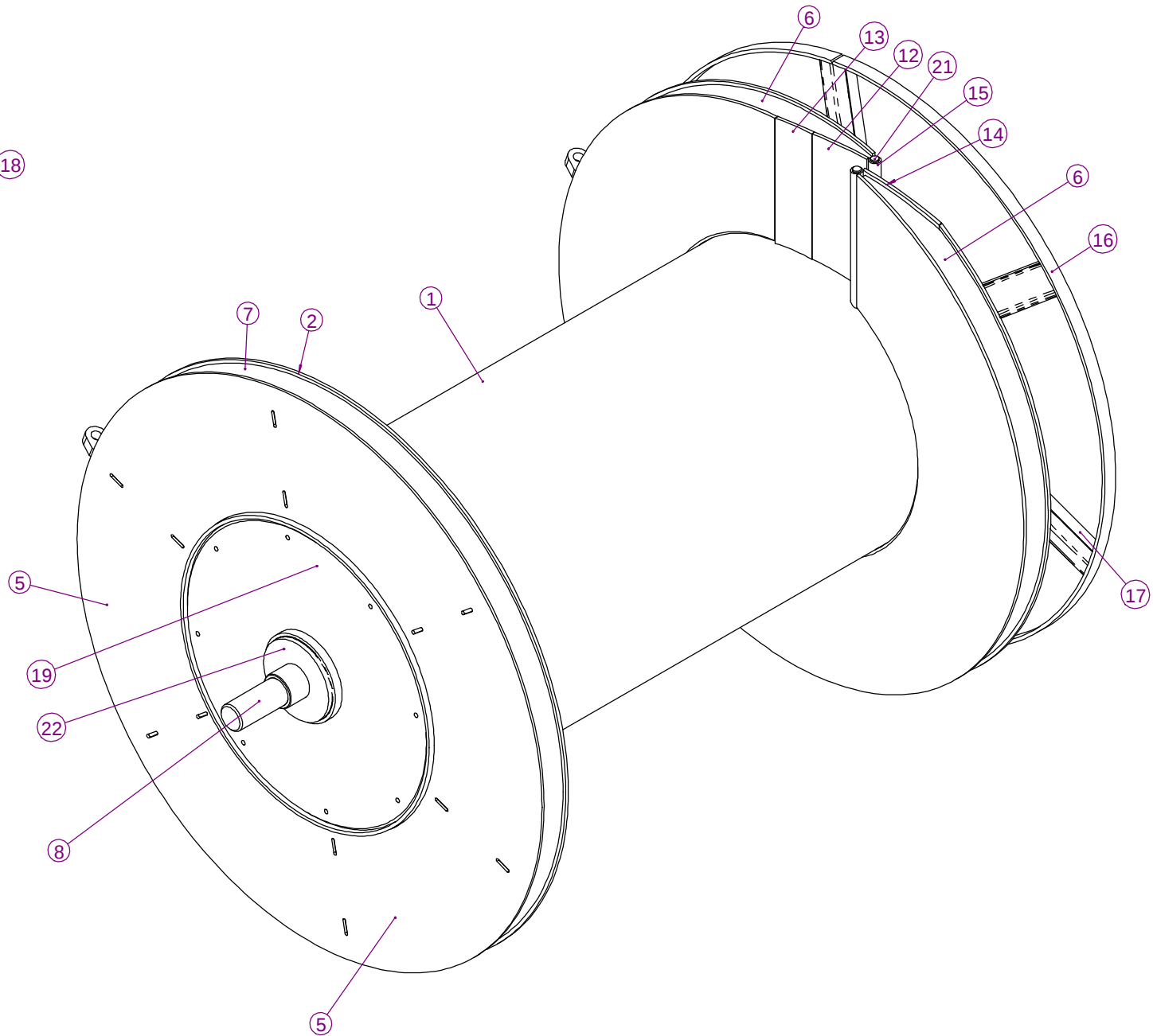
ISOMETRIC VIEWS
