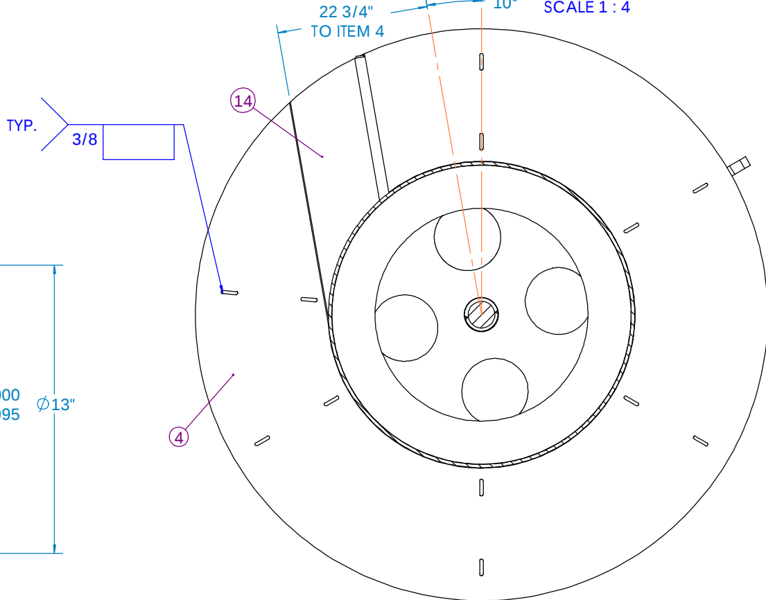
SECTION H-H
