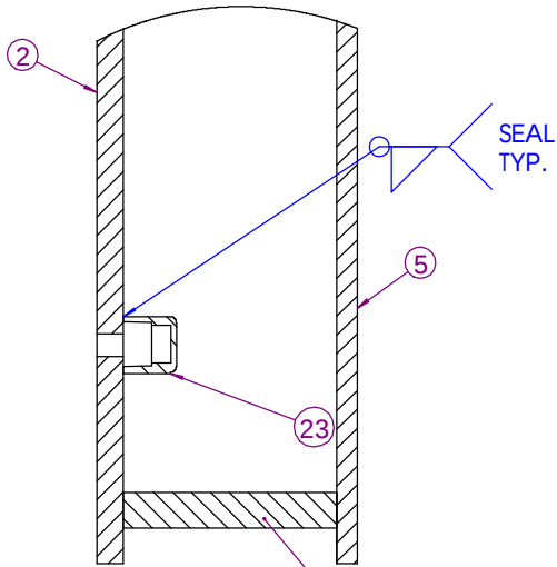
TYP. 12 PLACES SECTION E-E SCALE 1 : 4
