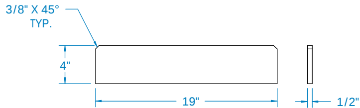
DETAIL ITEM 21 SCALE 1: 5 MAT'L: C. S. A-36 WT: 11 (12 REQ'D)
