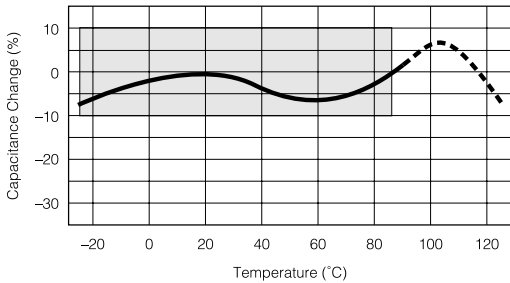
Char. B/Y5P
