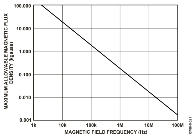
Figure 19. Maximum Allowable External Magnetic Flux Density
