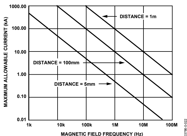
Figure 20. Maximum Allowable Current for Various Current-to-ADuM140x Spacings
