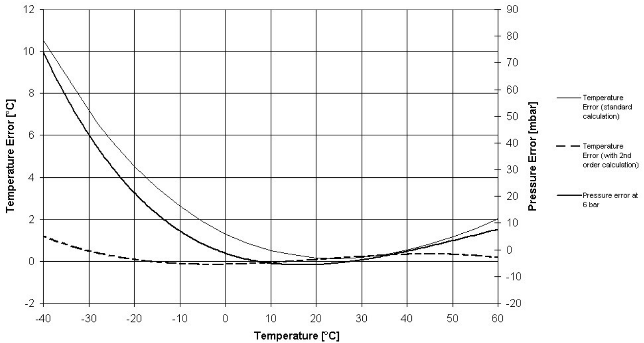
Accuracy vs temperature (typical)
