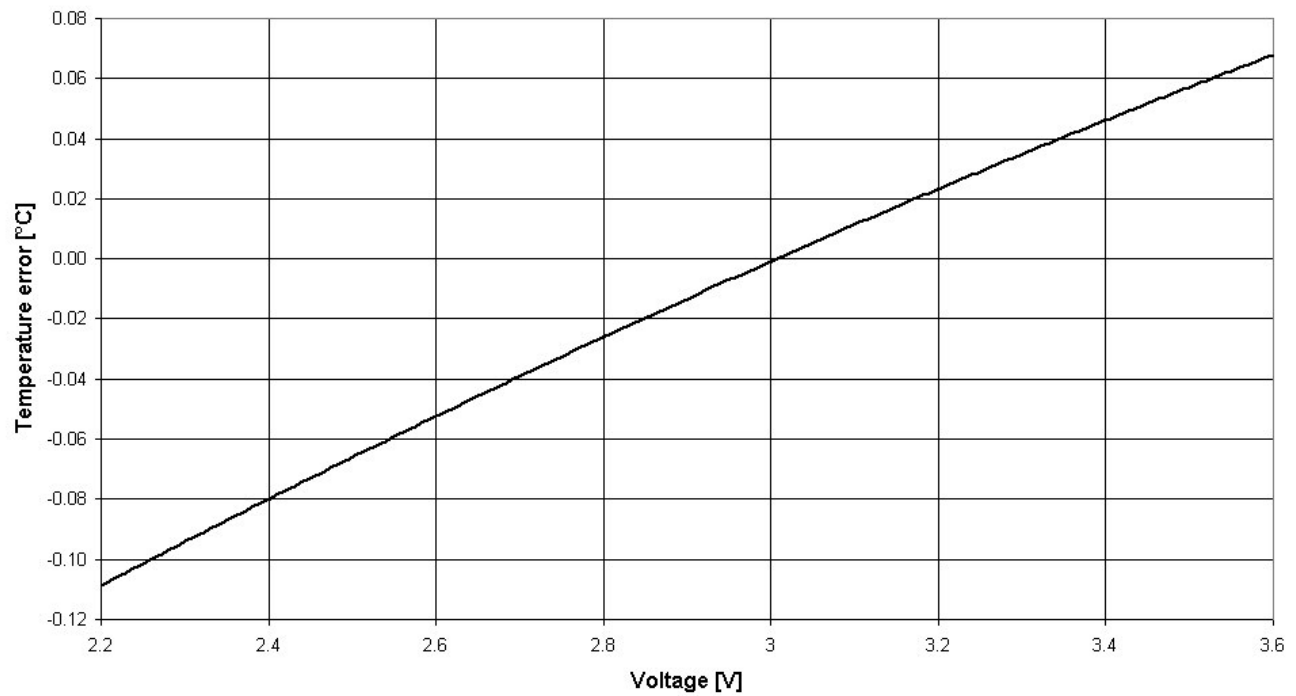
Temperature error (25°C) vs supply voltage (typical)
