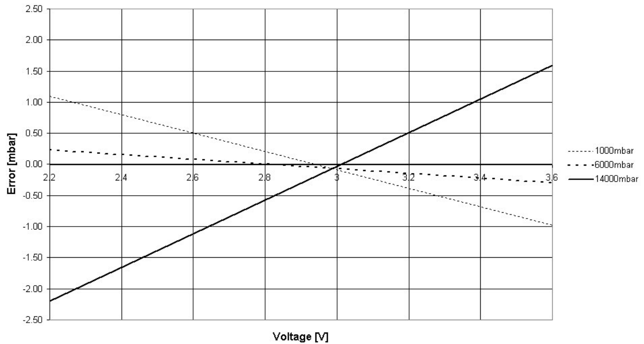
Pressure error vs supply voltage (typical)
