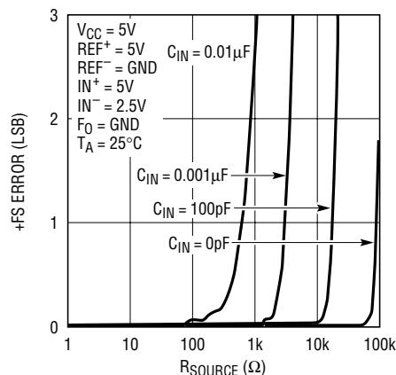
Figure 14. +FS Error vs R_{SOURCE} at \text{IN}^+ or \text{IN}^- (Small C_{IN} )
