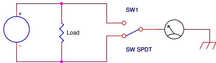
Floating Ammeter Concept
