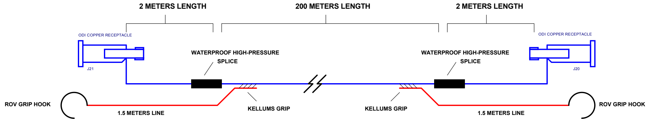
MECHANICAL ASSEMBLY
