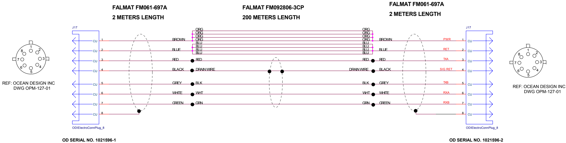
ELECTRICAL ASSEMBLY
