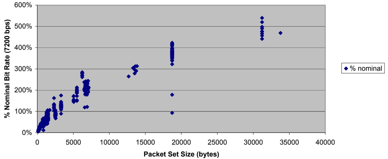
% Nominal Bit Rate vs Packet Set Size Globalstar Weekend Test
