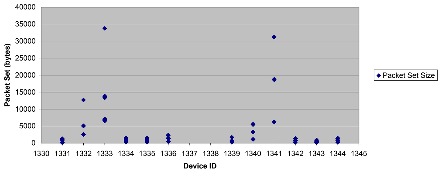
Packet Set Size vs Device ID Globalstar Weekend Test
