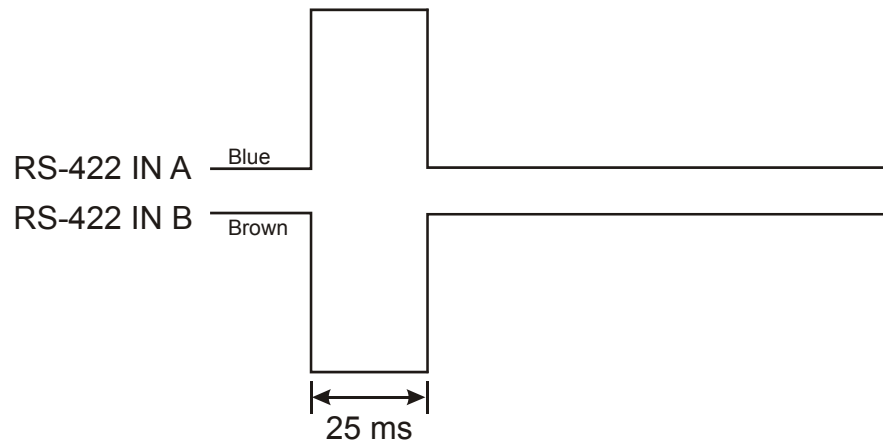
Figure 3. Timing Pulse
