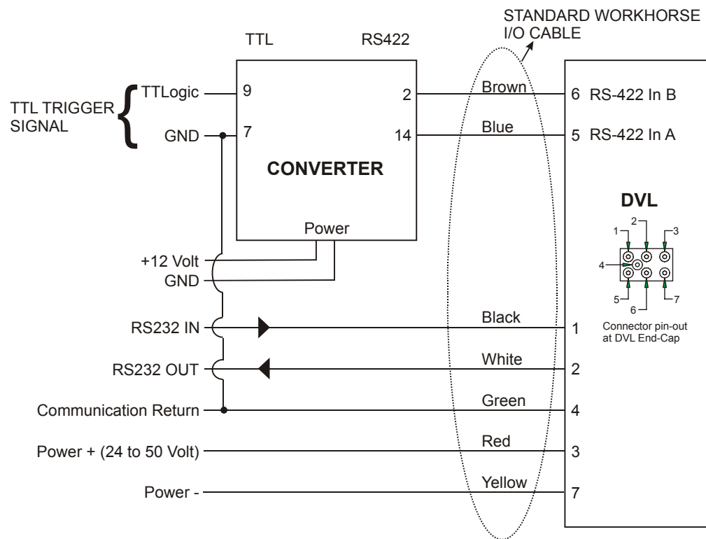
Figure 2. Triggering a DVL with a TTL Signal
