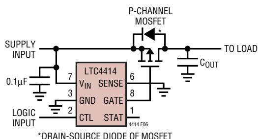
Figure 6. Logic Controlled High Side Power Switch
