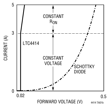
LTC4414 vs Schottky Diode Forward Voltage Drop
