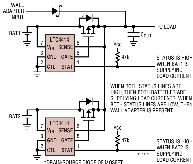
Figure 4. Dual Battery Load Sharing with Automatic Switchover of Load from Batteries to Wall Adapter
