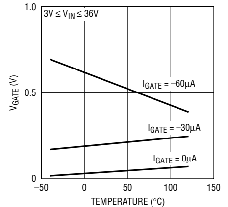
V_{G(OFF)} vs Temperature and I_{\text{GATE}}
