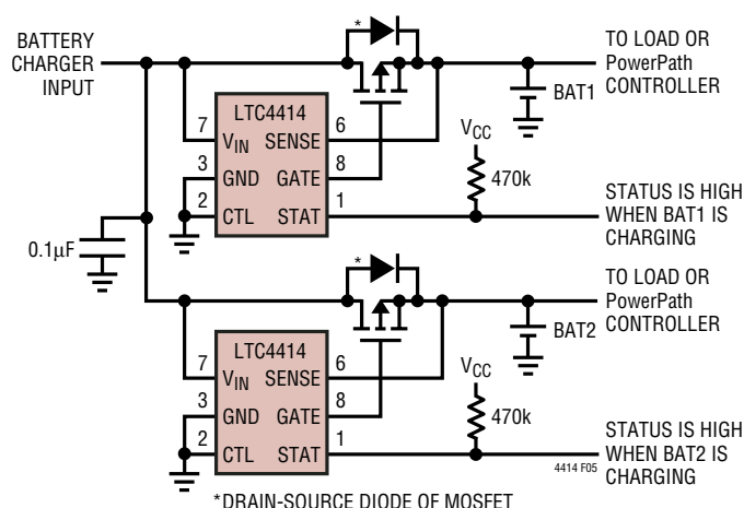
Figure 5. Automatic Dual Battery Charging from Single Charging Source
