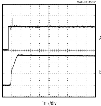
MAX5033BUSA STARTUP WAVEFORM ( I_O = 0 )
