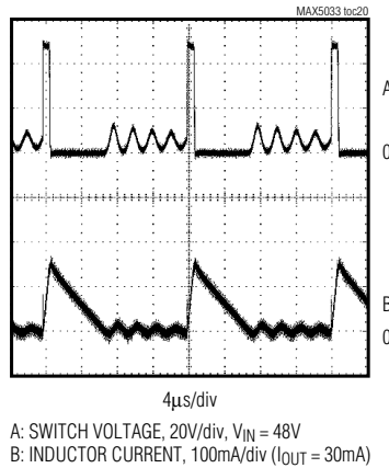
MAX5033BUSA LX WAVEFORMS
