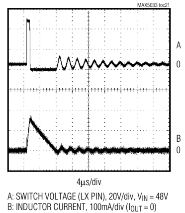
MAX5033BUSA LX WAVEFORMS
