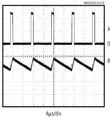
MAX5033BUSA LX WAVEFORMS
