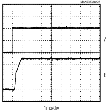
MAX5033BUSA STARTUP WAVEFORM ( I_O = 0.5A )
