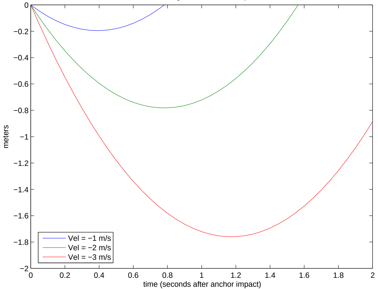
Landing Transient of Termination after Anchor Touchdown Inertial Considerations only, Drag neglected m = 800 \text{ kg} , 1.7 \text{ m} \times 0.9 \text{ m} ellipsoid
