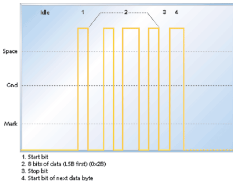
Figure 1: RS-232
