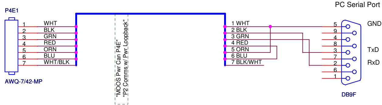
TEST CABLE FOR POWER CAN P2 SERIAL PORT, WITH POWER LOOPBACK
