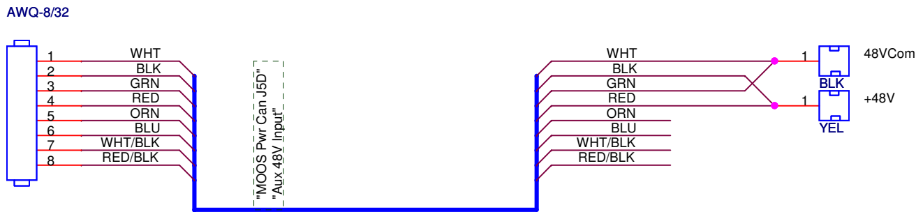
TEST CABLE FOR POWER CAN AUX PWR INPUT (OR LOAD SINK)
