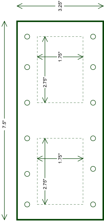
Power Can version -- keep components within dashed areas. Max height 1.75."
