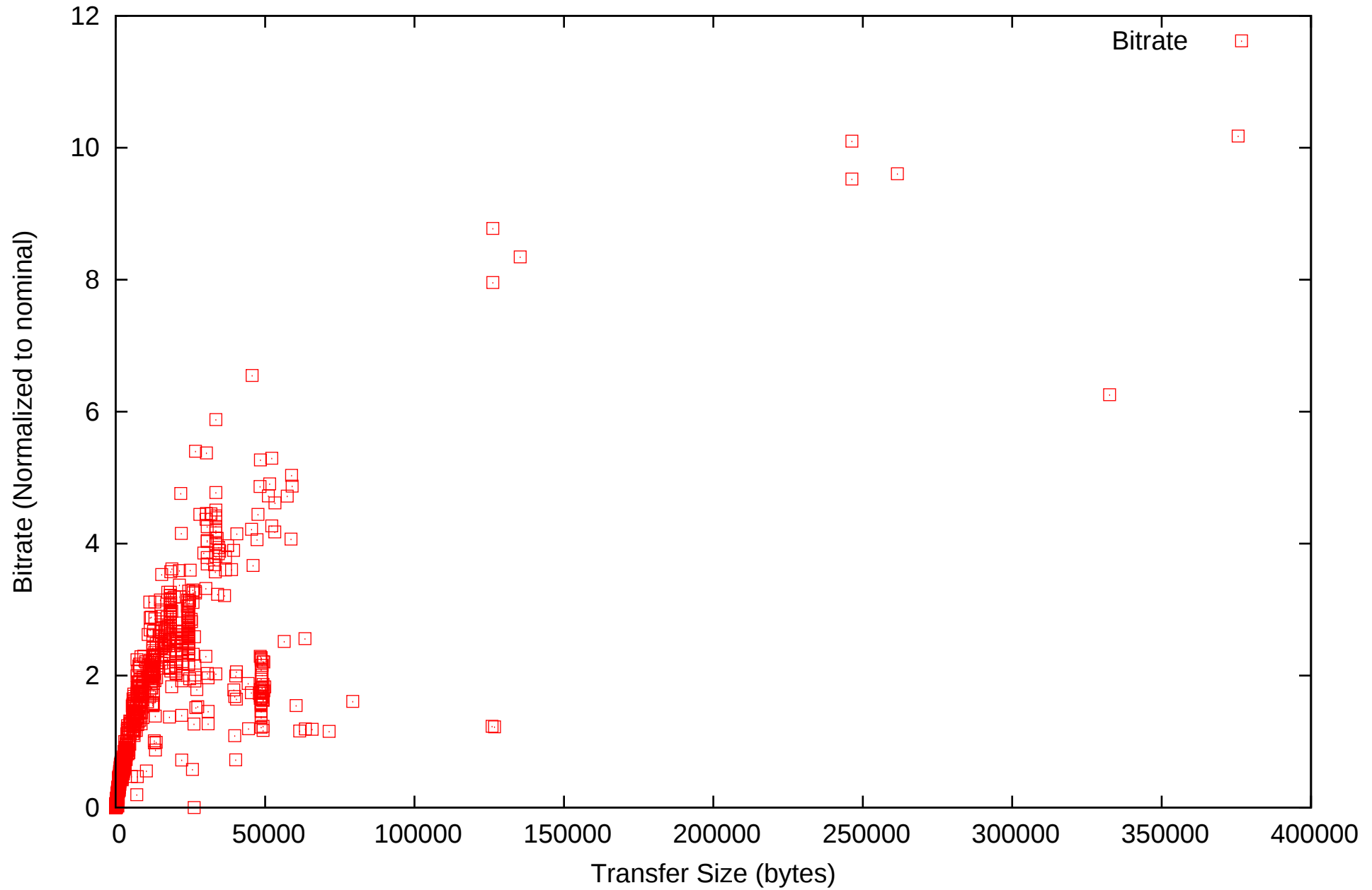
Bitrate vs Transfer Size
