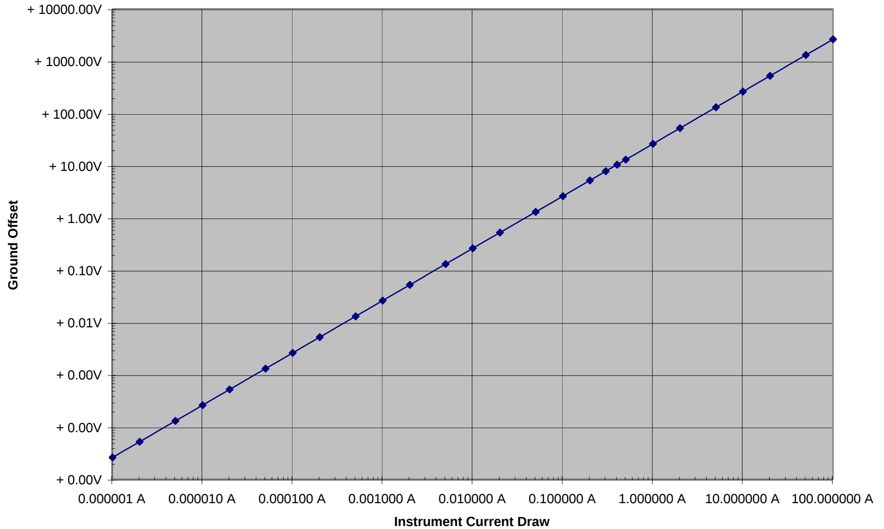
Instrument Ground Offset relative to Supply Ground - 1000m Benthic Instrument Cabling
