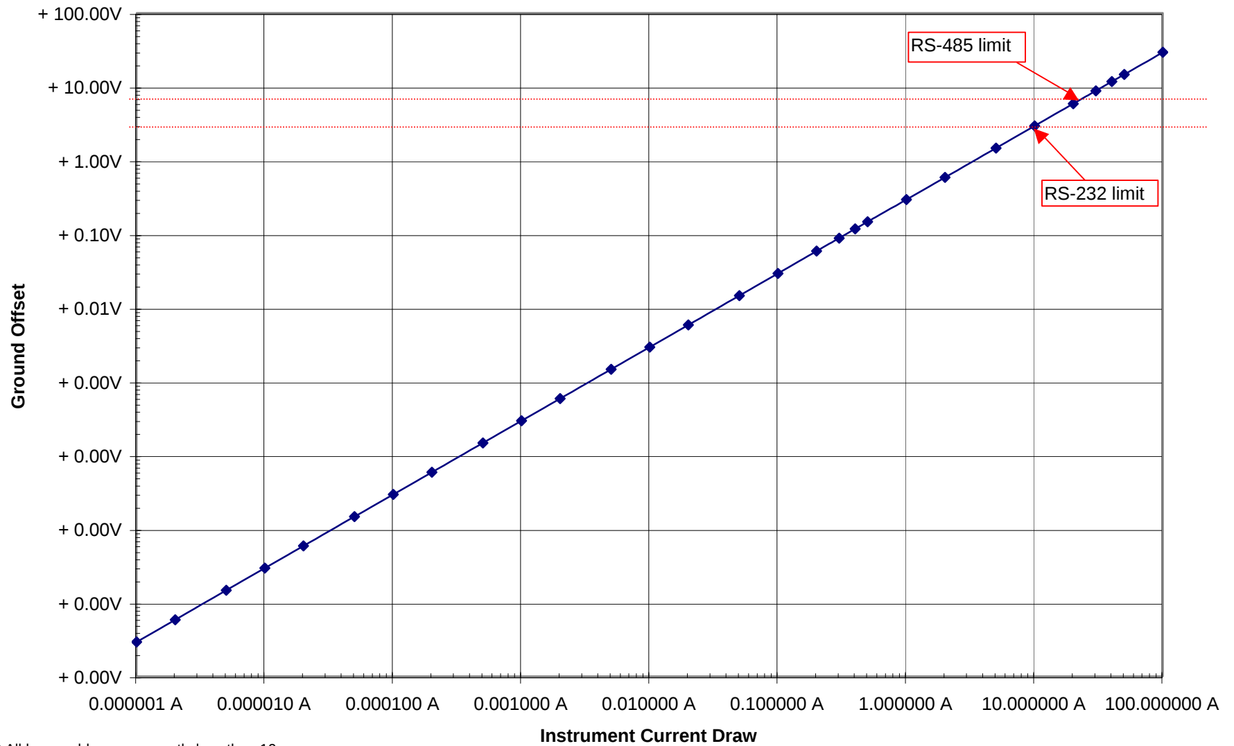
Instrument Ground offset relative to Supply Ground - 10m long* Buoy Cabling
