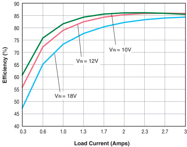
UWR-5/3000-D12A Efficiency vs. Line and Load
