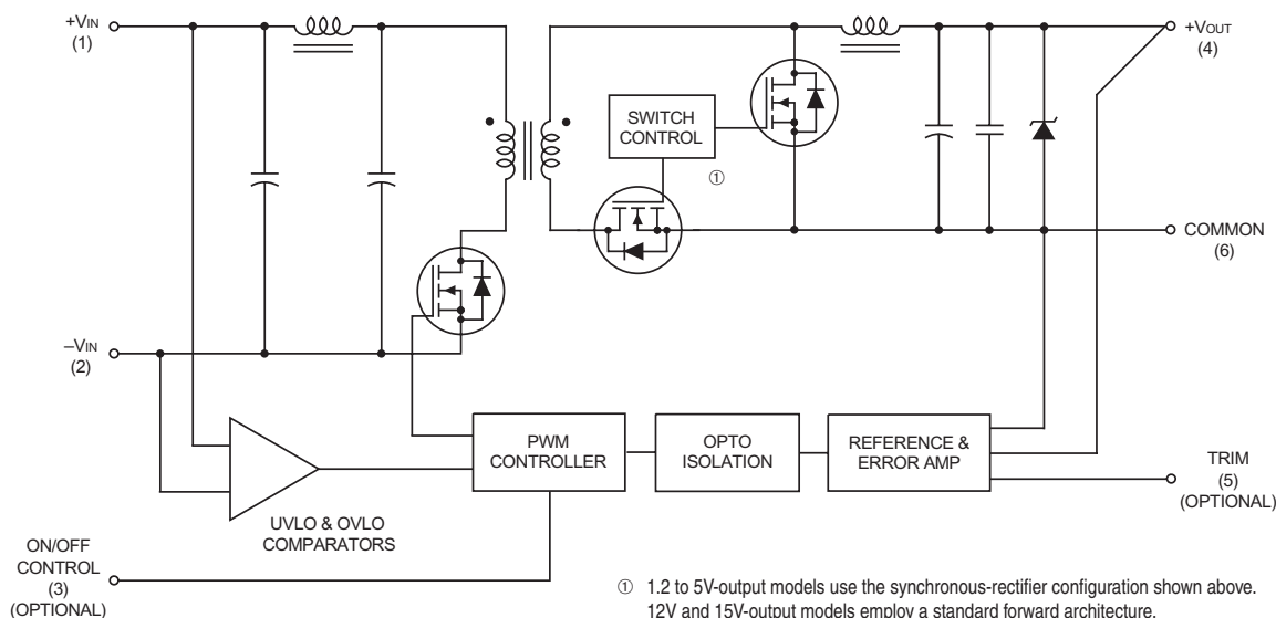
Figure 1. Simplified Schematic
