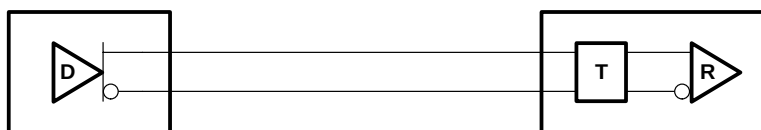
Figure 6. Point-to-Point Configuration
