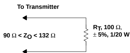
Figure 9. Differential Termination
