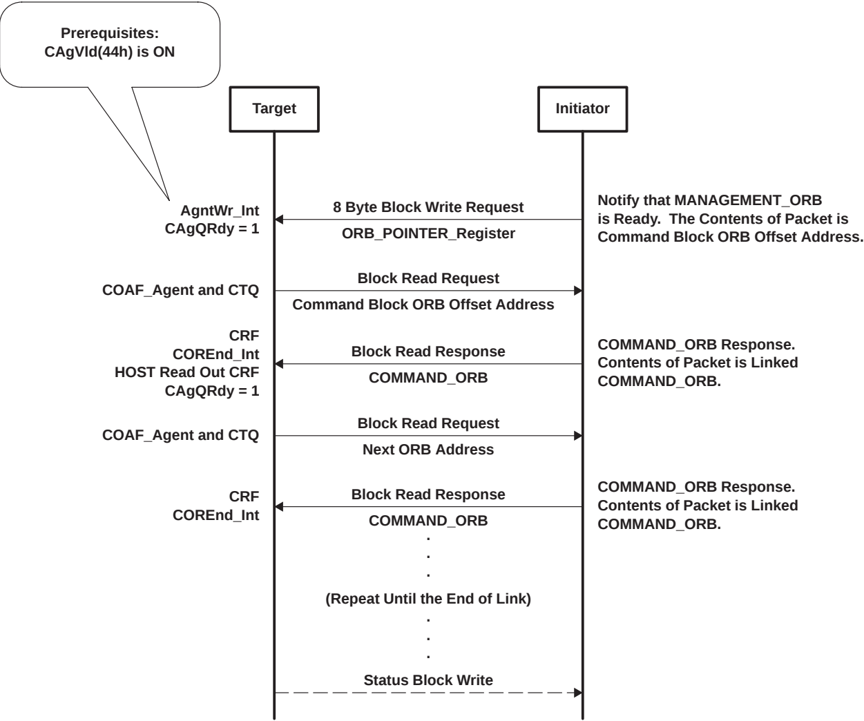
Figure 7-4. Typical Link Fetch
