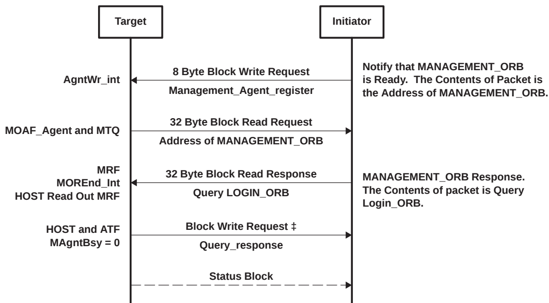
Figure 7–2. Typical Management ORB Transaction
