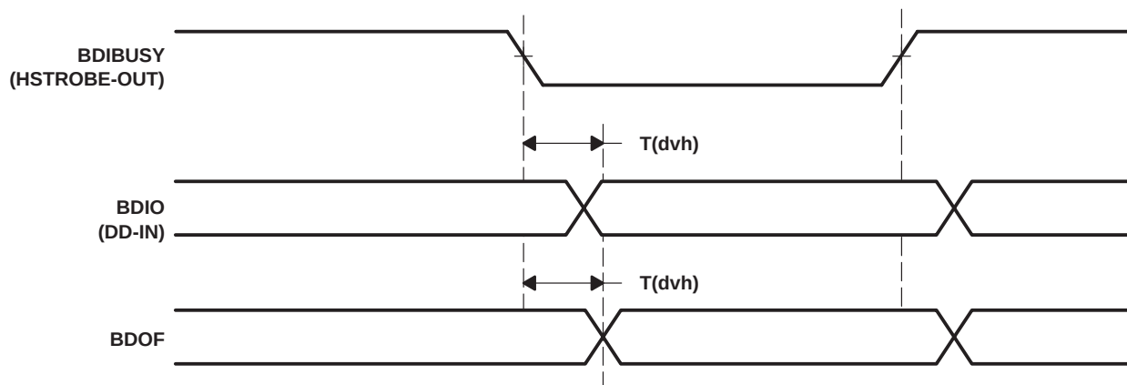
Figure 9–13. ATAPI Write
