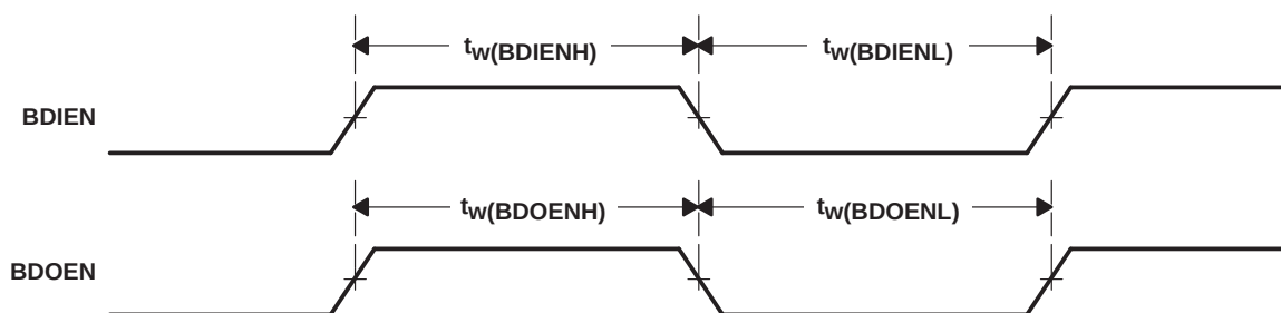
Figure 9-4. Asynchronous Mode
