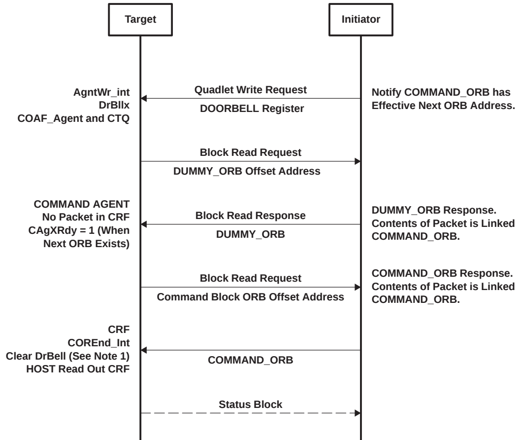
Figure 7-5. SUSPENDED and DOORBELL Request by DUMMY ORB
