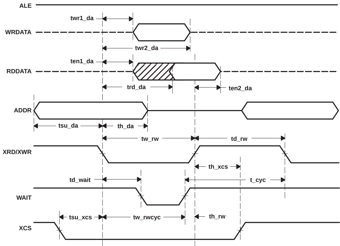
Figure 10–1. Parallel Mode Read/Write Cycle
