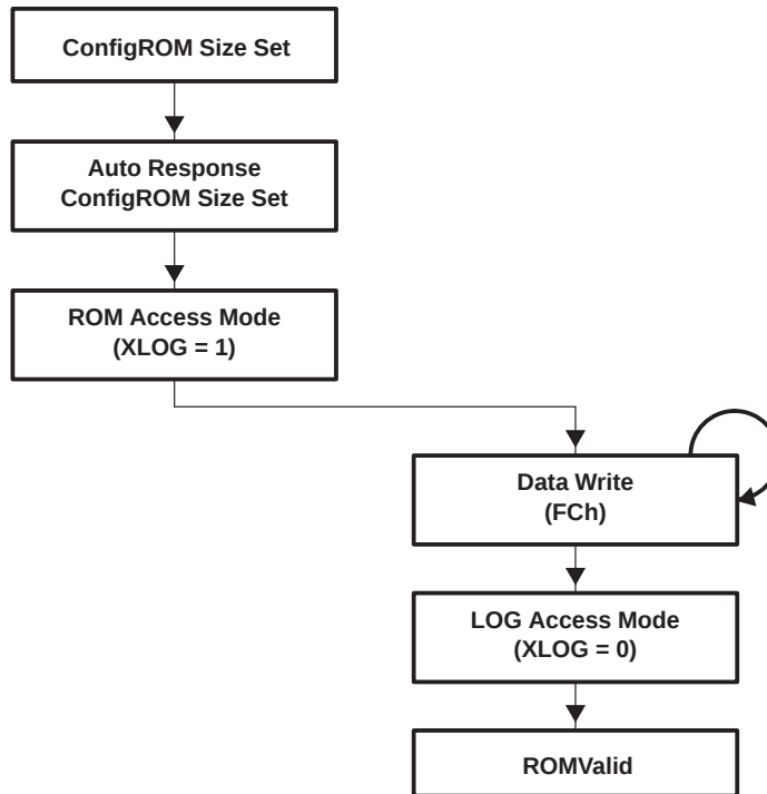
Figure 5-2. Config ROM Setup
