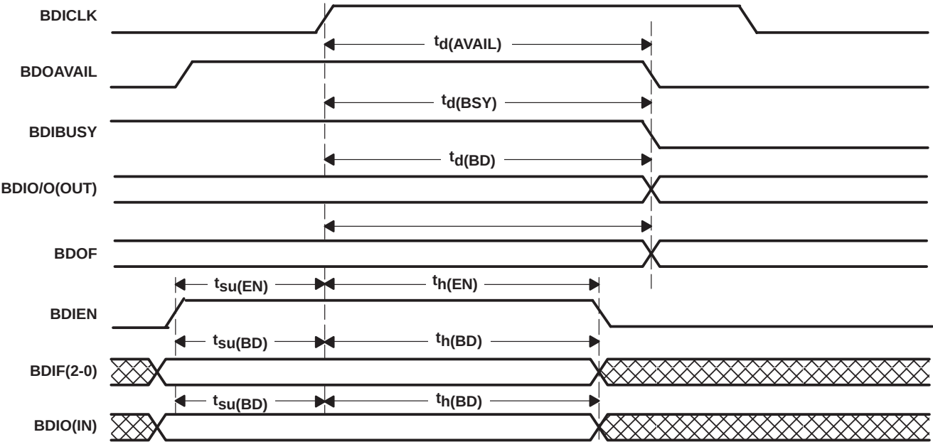
Figure 9–1. Synchronous Mode
