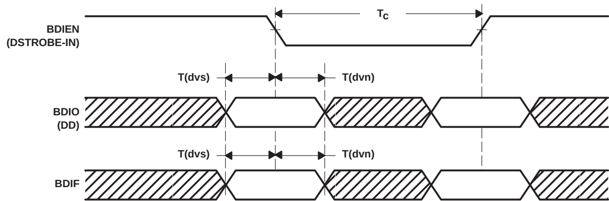
Figure 9-10. ATAPI Read
