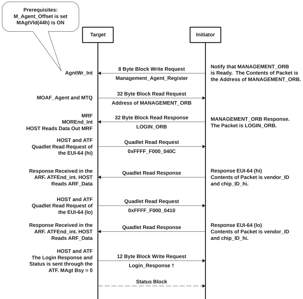
Figure 7–1. Typical LOGIN Process
