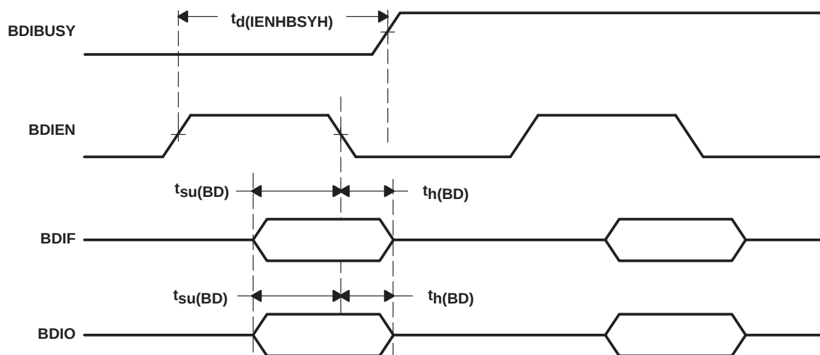
Figure 9-7. Asynchronous Burst Mode Write
