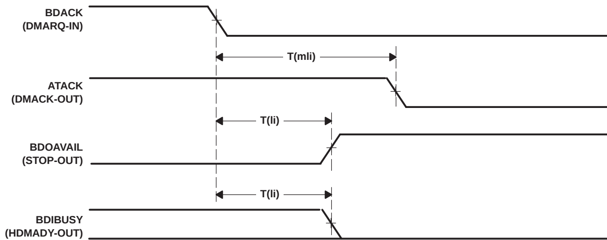
Figure 9-11. ATAPI Terminate (Read)
