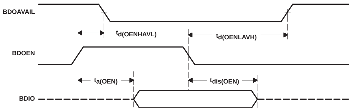
Figure 9-6. Asynchronous Handshake Mode Read
