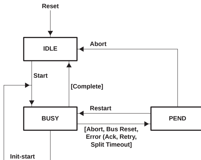
Figure 3–1. Automatically Creating a SBP-2 Compliant Request for a Block Packet
