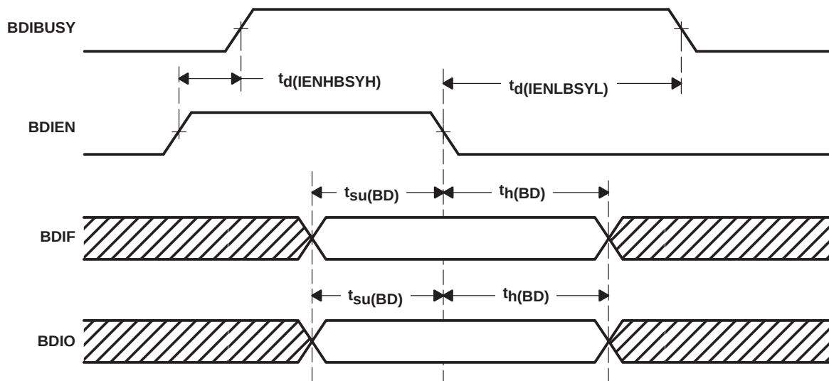
Figure 9-5. Asynchronous Handshake Mode Write
