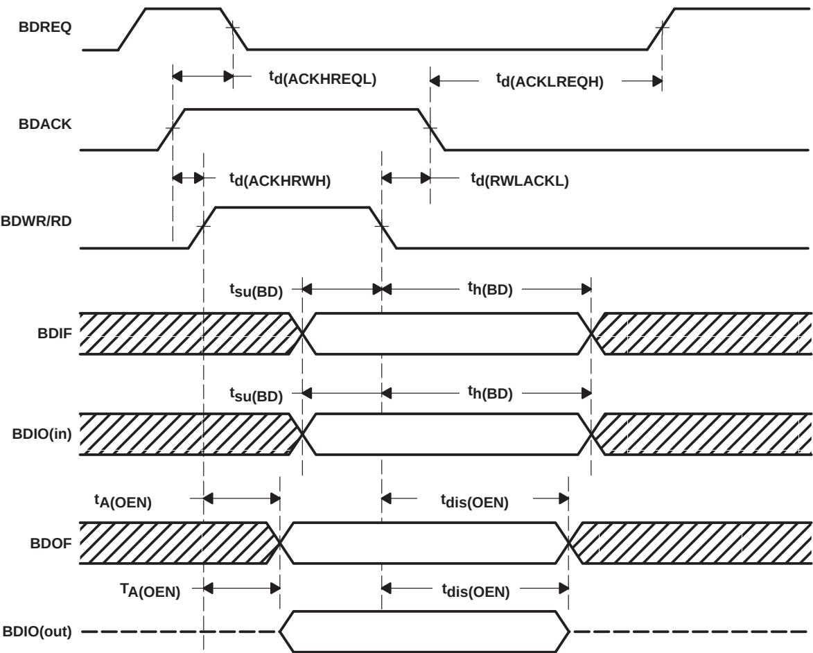
Figure 9-2. SCSI Handshake Mode
