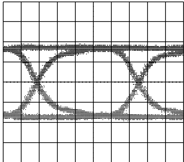
Timebase = 500 ps/div Ch. 1 = 200.0 mV/div Source Terminated Signal
