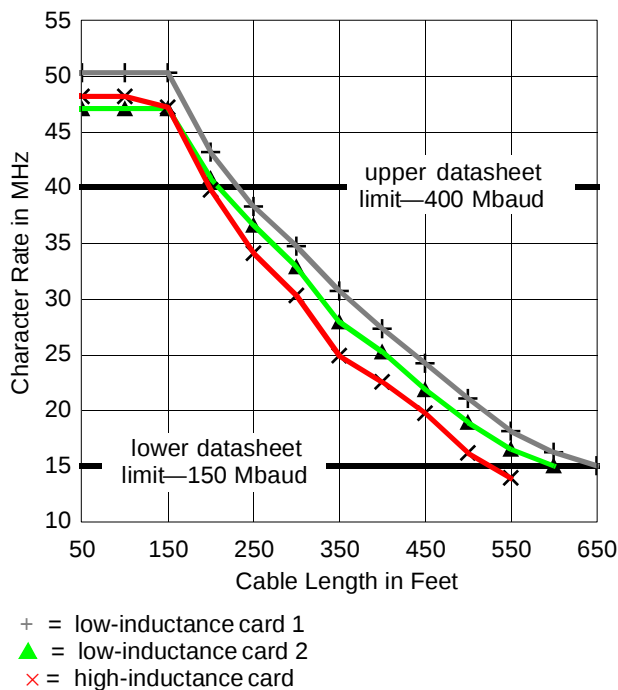
Figure 3. RG59 Test Results, Linear Frequency Scale
