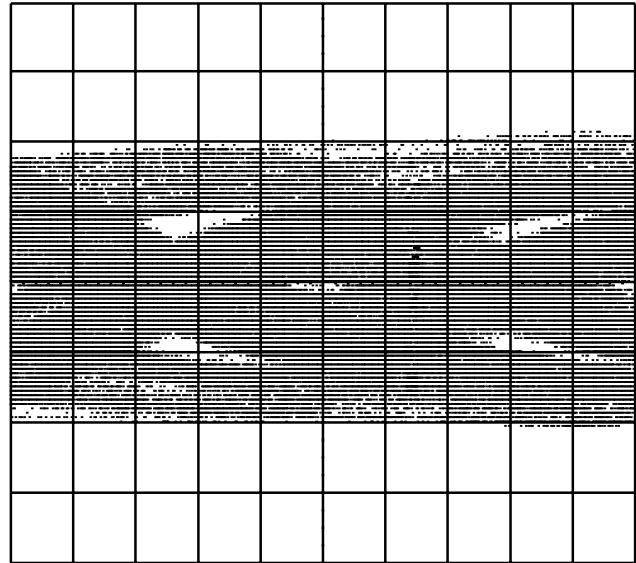
Timebase = 500 ps/div Ch. 1 = 100.0 mV/div Source Terminated Signal
