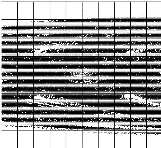
Timebase = 1.00 ns/div Ch. 1 = 100.0 mV/div Normal Signal
