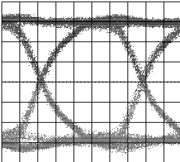
Timebase = 500 ps/div Ch. 1 = 200.0 mV/div Normal Signal
