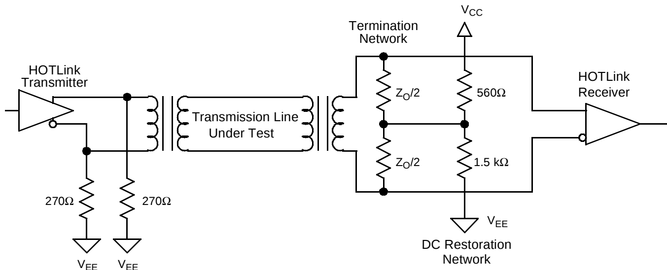
Figure 1. Cable Test Configuration
