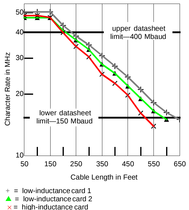
Figure 4. RG59 Test Results, Log Frequency Scale
