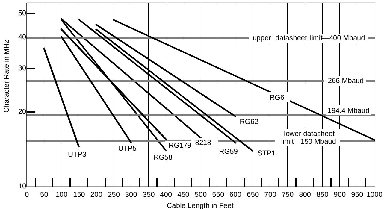
Figure 5. Maximum Data-Rate versus Distance Comparison
