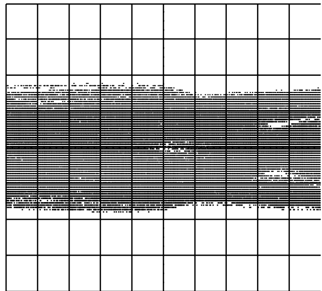
Timebase = 1.00 ns/div Ch. 1 = 100.0 mV/div Source Terminated Signal
