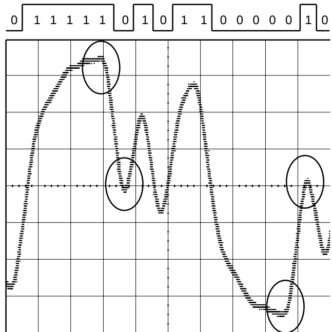
Timebase = 5.00 ns/div Ch. 1 = 100.0 mV/div 363 Mbits/second @ 550 Feet
