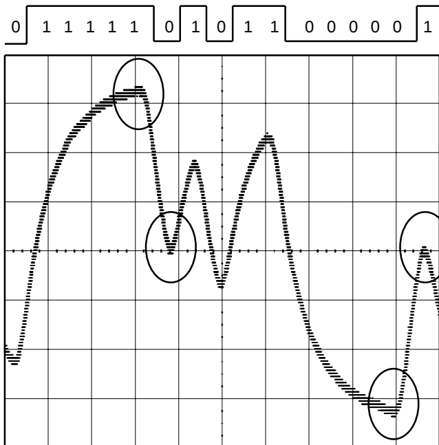
Timebase = 10.0 ns/div Ch. 1 = 100.0 mV/div 173 Mbits/second @ 550 Feet
