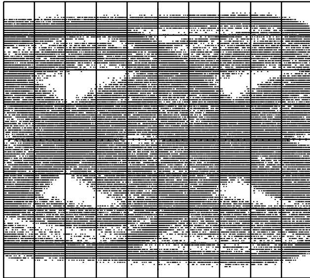
Timebase = 500 ps/div Ch. 1 = 100.0 mV/div Normal Signal
