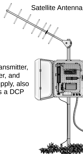
Data Collection Platform (DCP)
