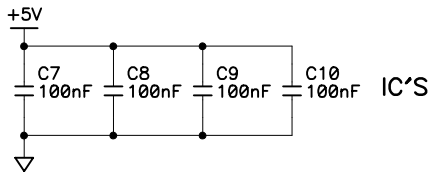
Decoupling Capacitors
