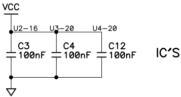
Decoupling Capacitors
