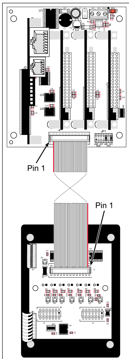
Figure B-7. Connecting LCD/Keypad Module to Backplane
