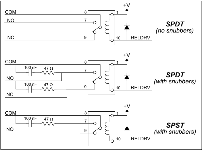
Figure 45. Relay Configurations
