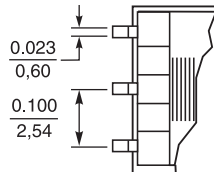
Terminal Dimensions
