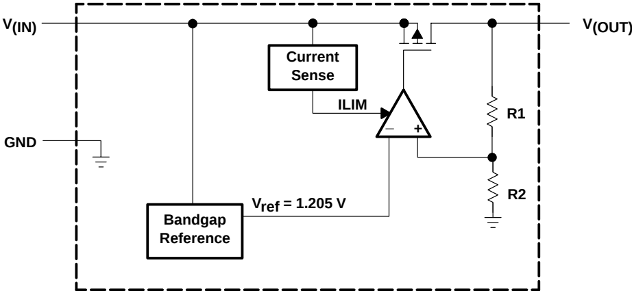
functional block diagram – fixed version
